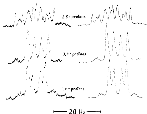
Figure 1. Experimental and calculated spectra, 7-( p -methoxyphenyl)-7-carbomethoxynorcaradiene-1,3,5-cycloheptatriene equilibrium mixture, CDCl 3 solution, 33°, 220 MHz, 100-Hz sweep width.
